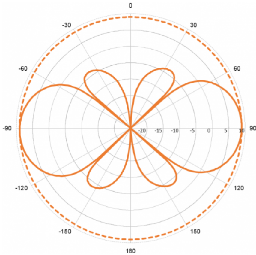
Radiation Pattern
