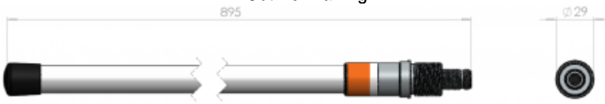
Outline Drawing
